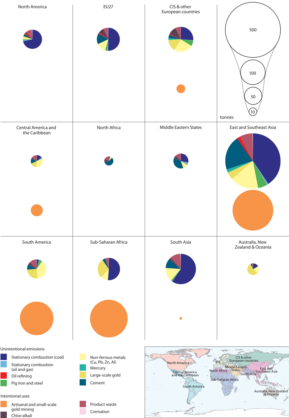
Estimates of 2010 anthropogenic mercury emissions to air from different main sectors in different regions. ASGM is shown separately to highlight its geographic distribution and better allow regional comparisons to be made for other sectors.
